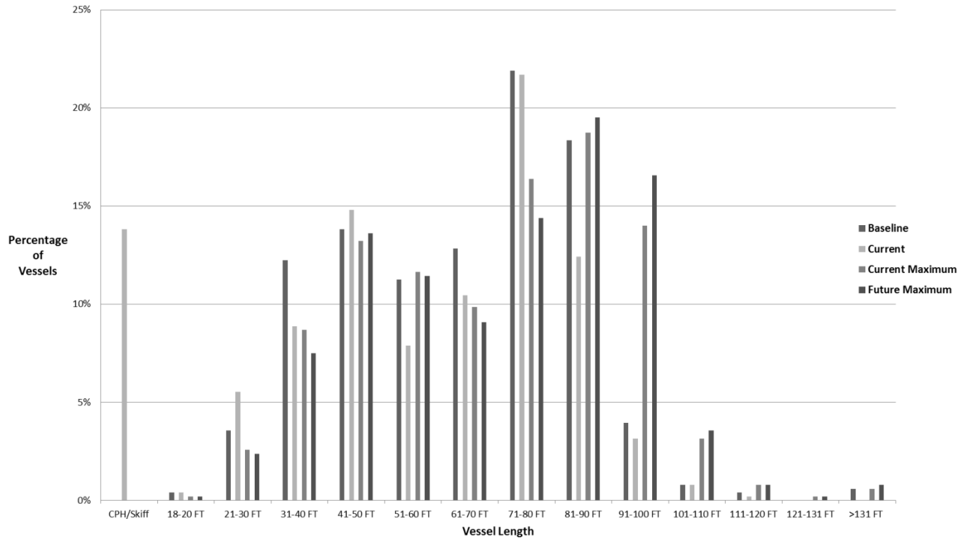
Figure 17. Mid-Atlantic Limited Access Vessel Size and Horsepower Frequency
