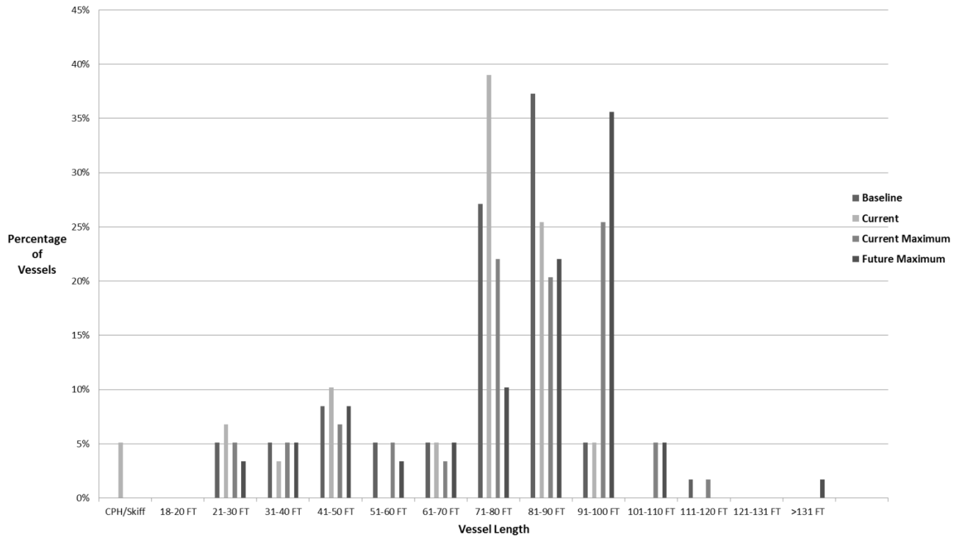
Figure 28. Virginia Limited Access Vessel Size and Horsepower Frequency
