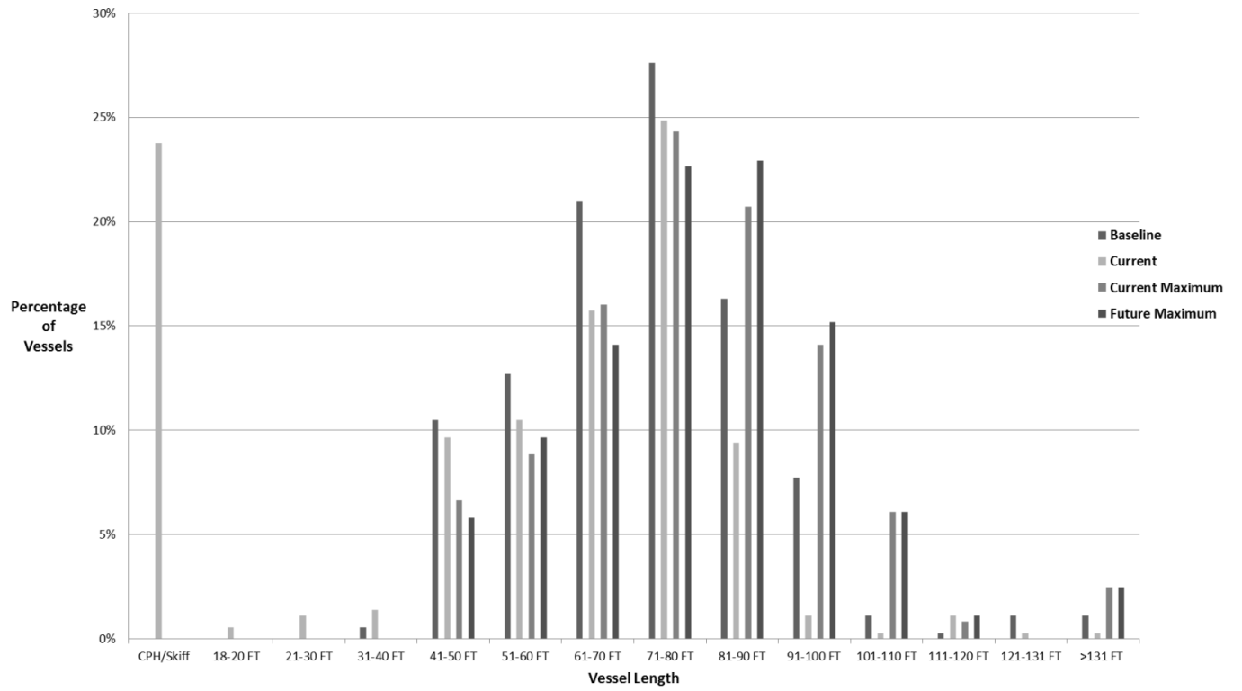
Figure 9. Limited Access Longfin Squid Vessel Size and Horsepower Frequency
