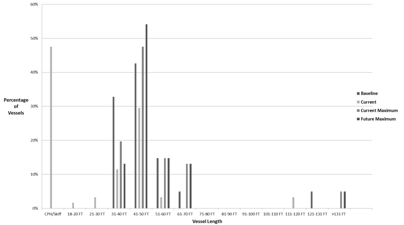
Figure 19. New Hampshire Limited Access Vessel Size and Horsepower Frequency
