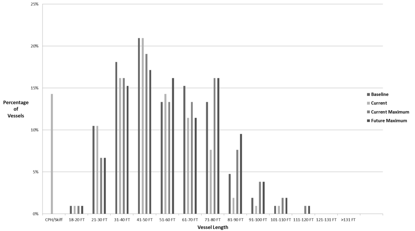
Figure 23. New York Limited Access Vessel Size and Horsepower Frequency
